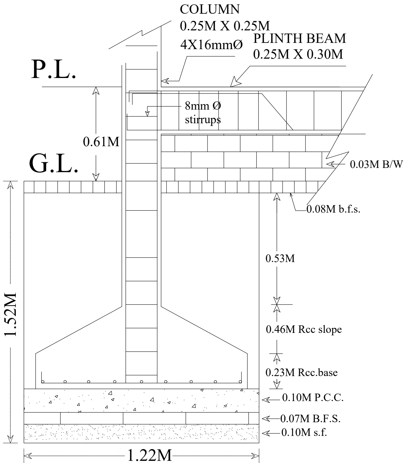
C/S OF EXSISTING.FOOTING
