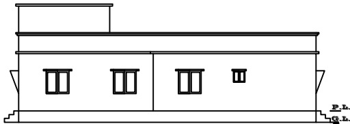
SIDE ELEVATION
