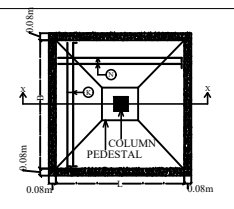
PLAN OF ISOLATED FOOTING
