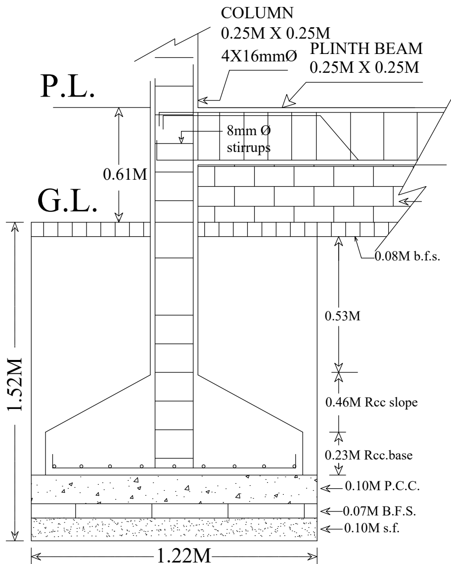
C/S OF FOOTING
