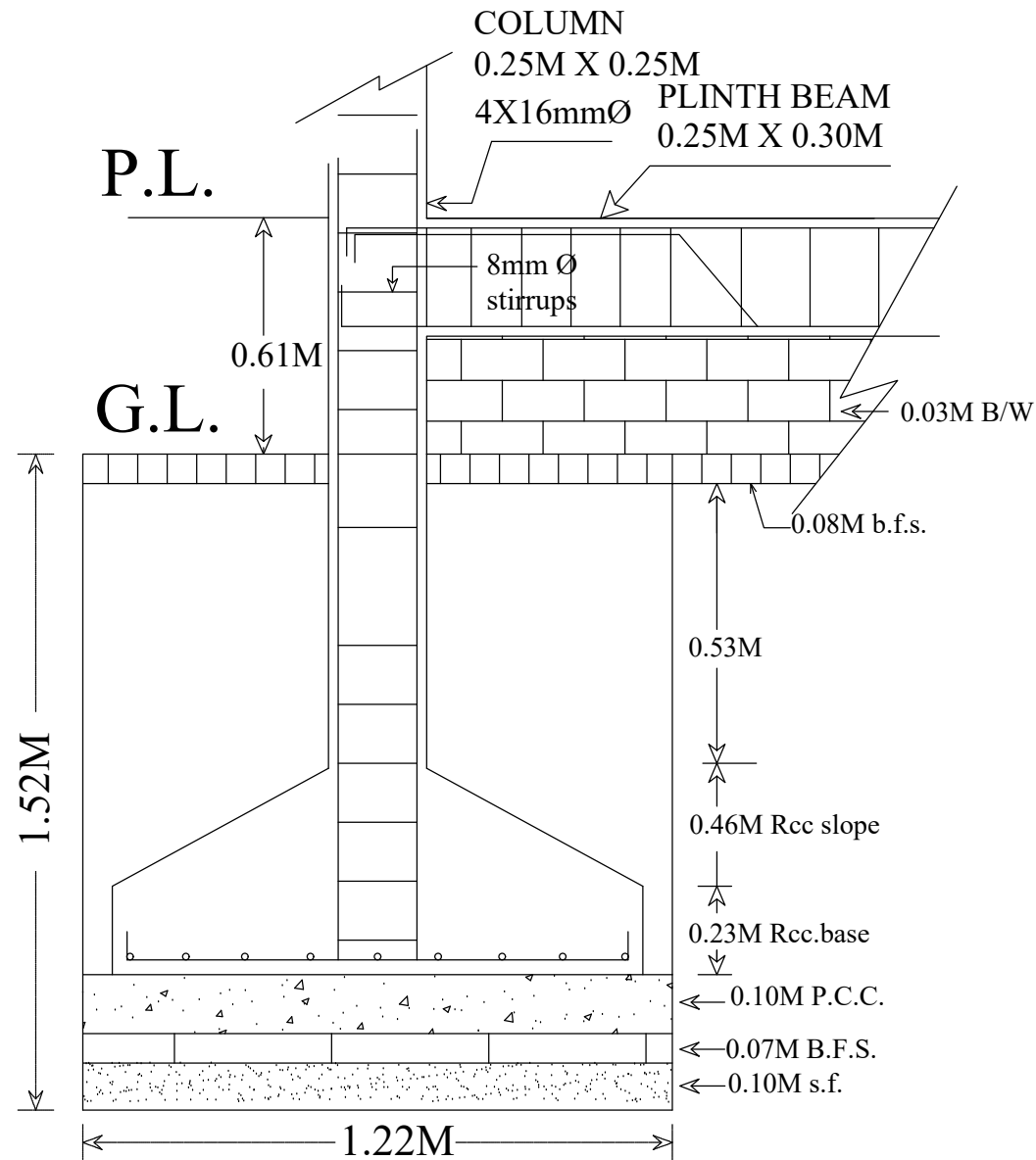
C/S OF FOOTING
