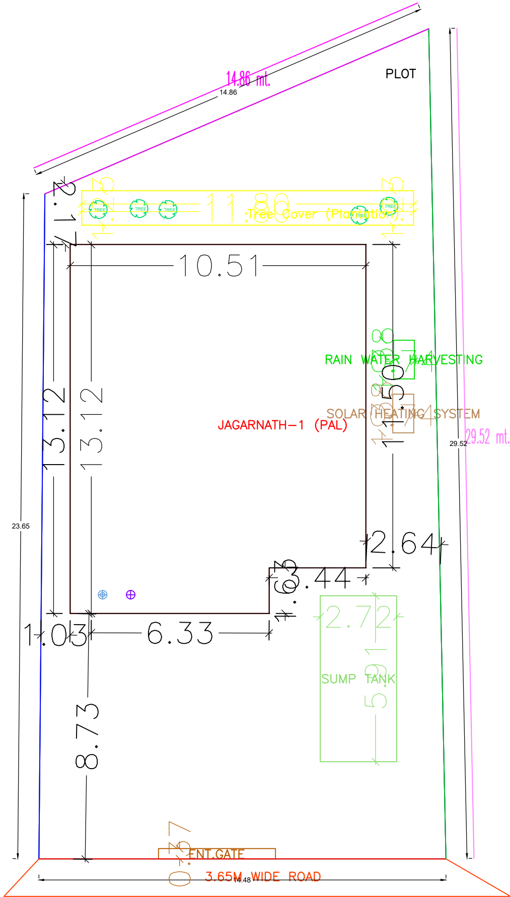
SITE PLAN
