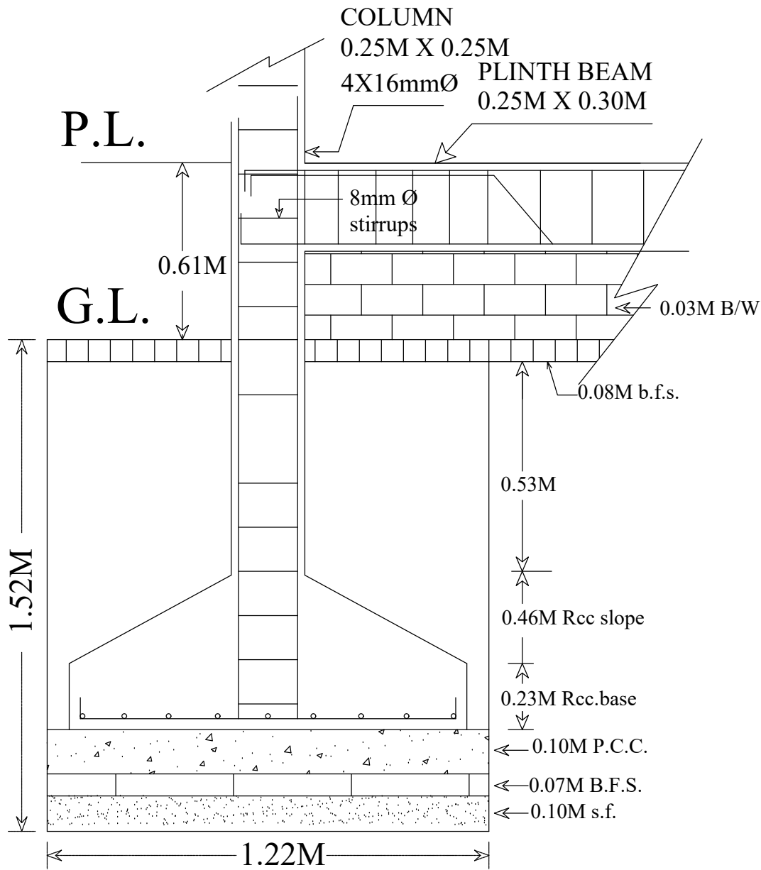
C/S OF EXSISTING FOOTING
