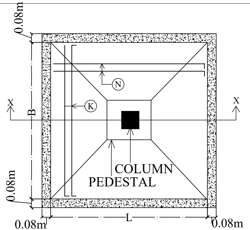
PLAN OF EXSISTING ISOLATED FOOTING
