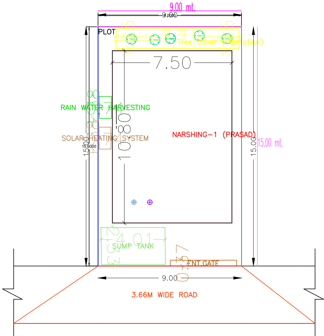
SITE PLAN
