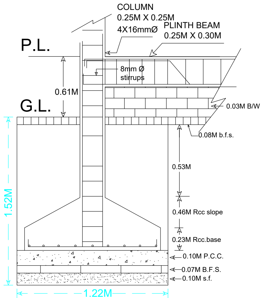
C/S OF FOOTING
