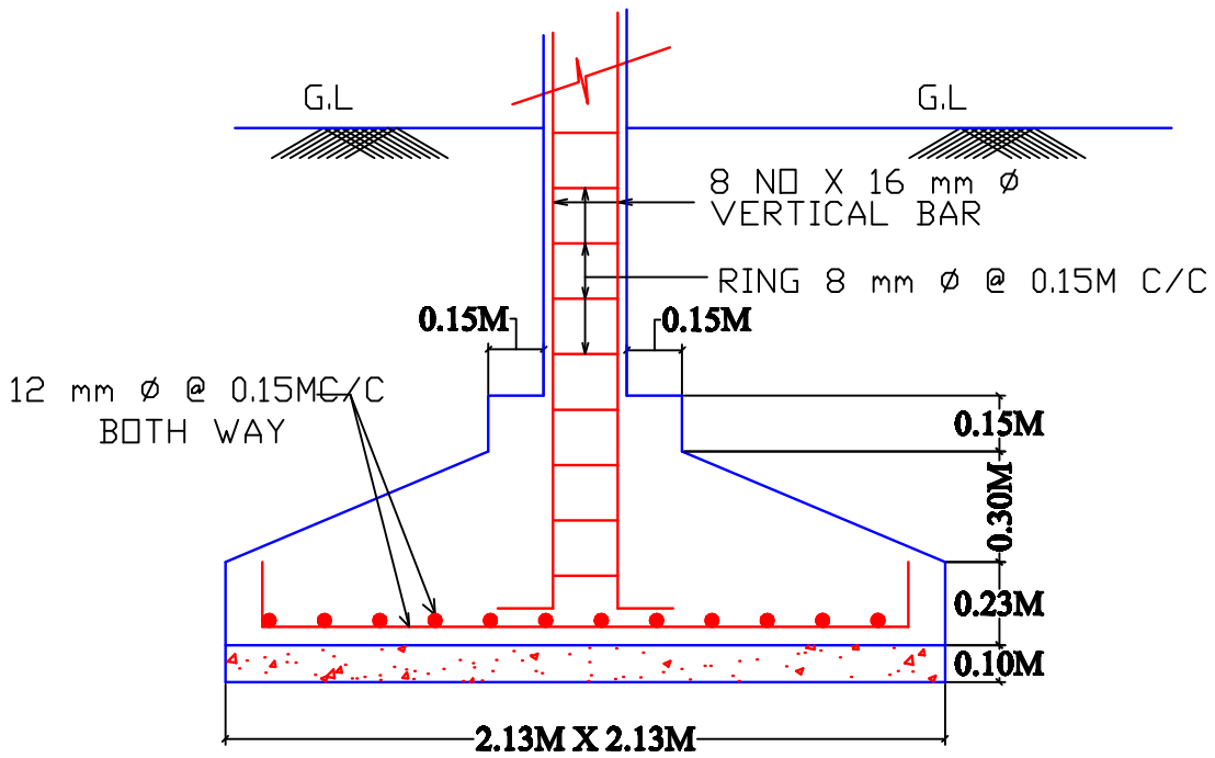
SECTION OF FOOTING . SIZE - 2.13M X 2.13M
