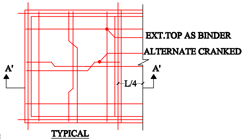
SECTION OF FOOTING . SIZE - 2.13M X 2.13M
