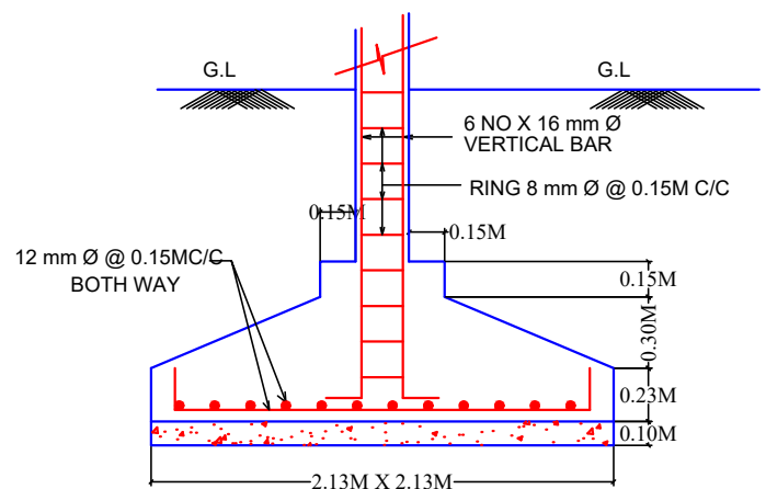
SECTION OF FOOTING SIZE - 2.13M X 2.13M
