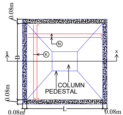
PLAN OF ISOLATED FOOTING
