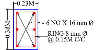
C.S. OF COLUMN SIZE - 0.23M X 0.38M
