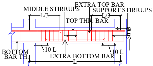
SECTION OF TYPICAL FLOOR BEAM
