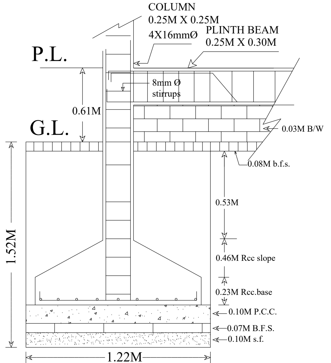
C/S OF FOOTING
