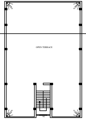
TERRACE FLOOR PLAN SCALE: 1:100
