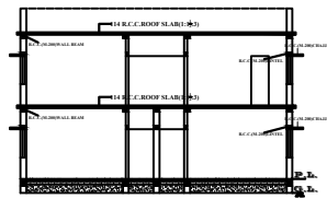
C/S AT A-A
