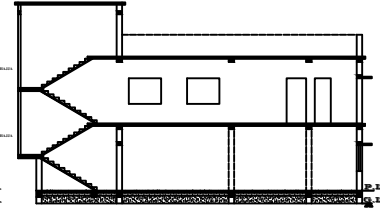
C/S AT B-B
