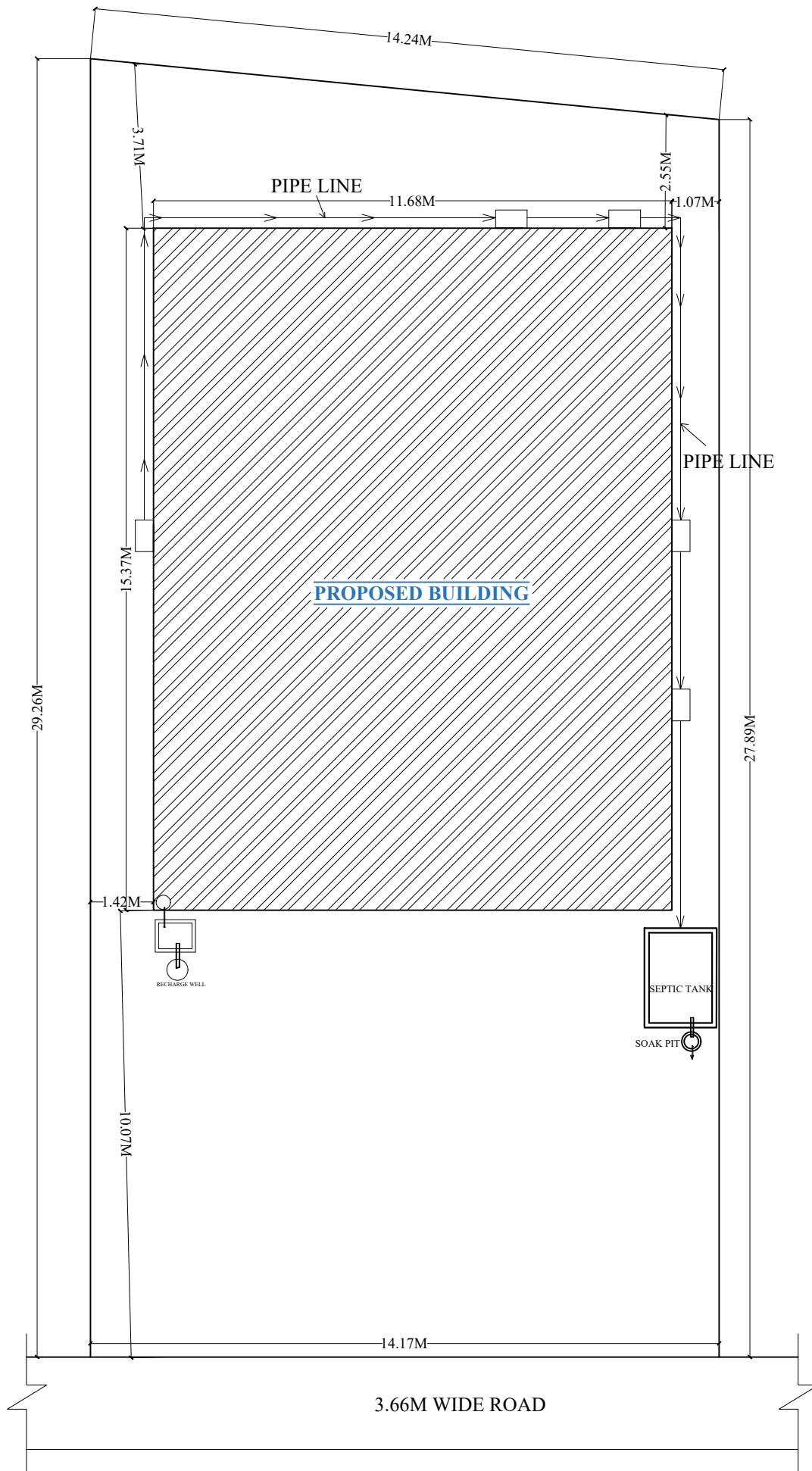
NORTH SIDE ROAD & FRONT SCALE : 1:100 KEY PLAN
