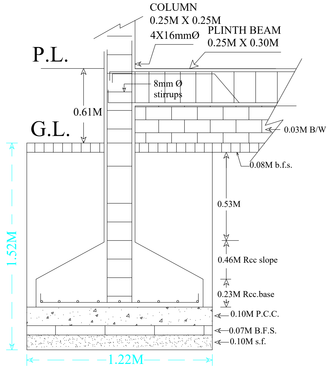
C/S OF FOOTING
