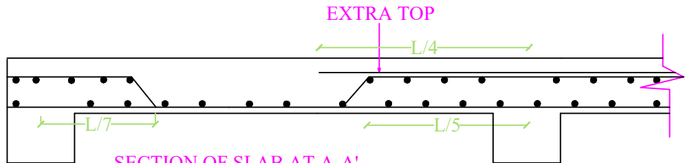
SECTION OF SLAB AT A-A'
