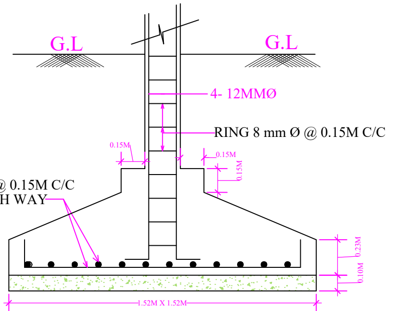
SECTION OF FOOTING .
