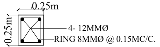
SECTION OF COLUMN.
