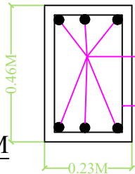
SECTION OF COLUMN.
