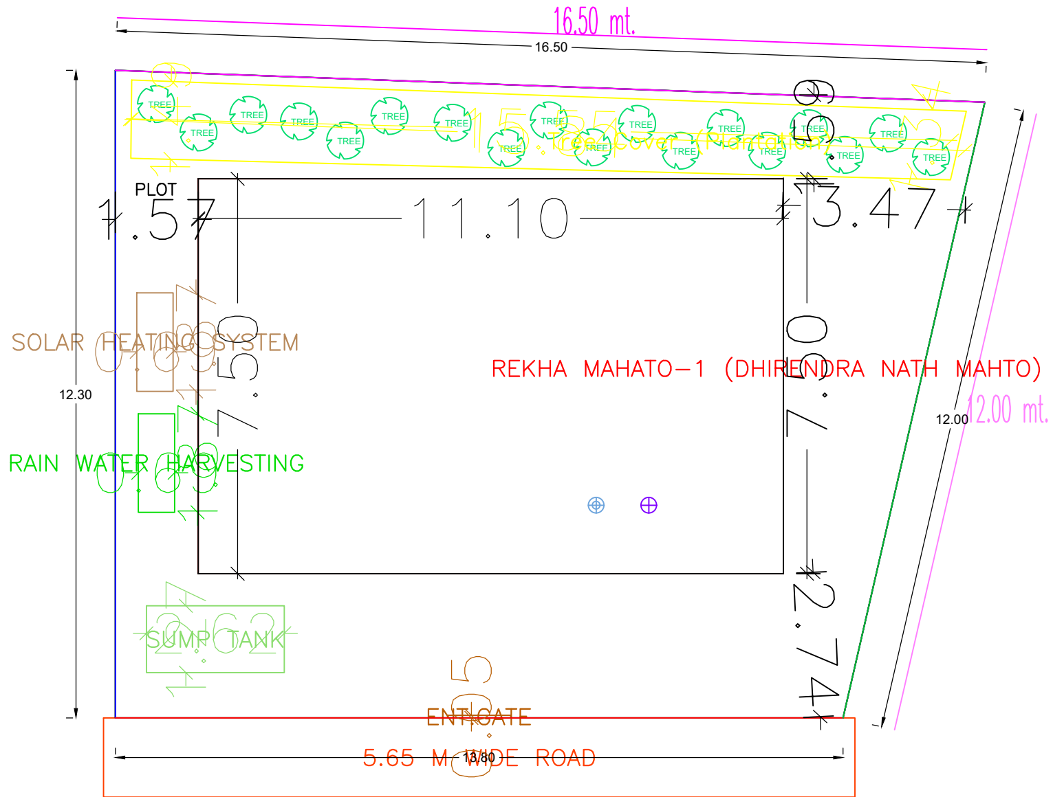
SITE PLAN
