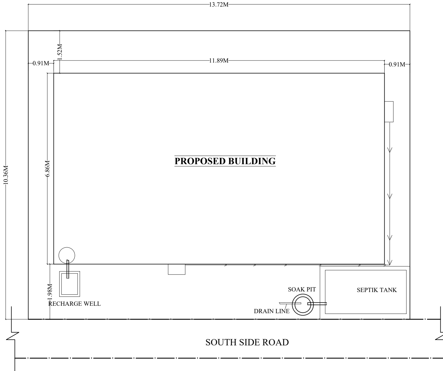
KEY PLAN NORTH SIDE ROAD & FRONT SCALE-1:100
