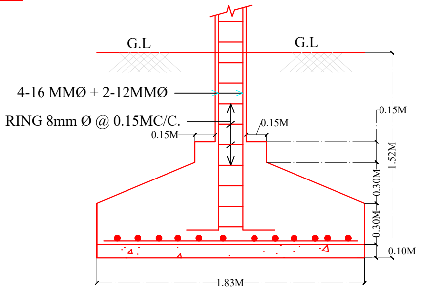
SECTION OF FOOTING
