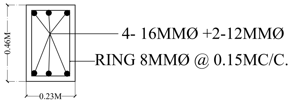
SECTION OF COLUMN.
