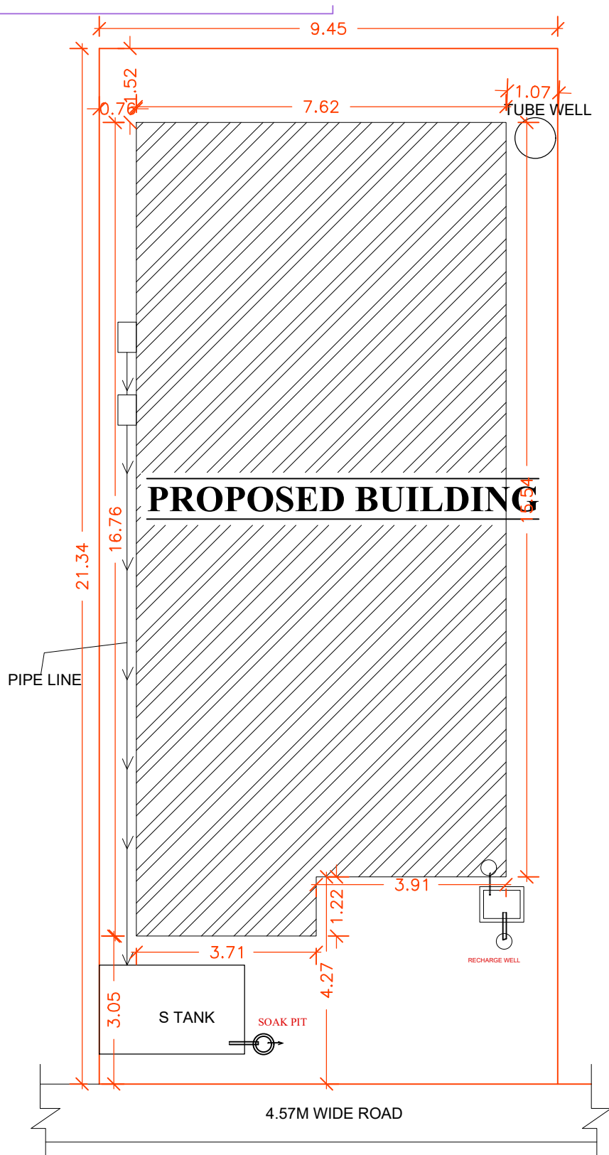
SOUTH SIDE ROAD & FRONT SITE PLAN SCALE-1:100
