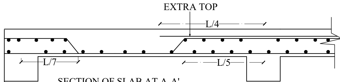
SECTION OF SLAB AT A-A'
