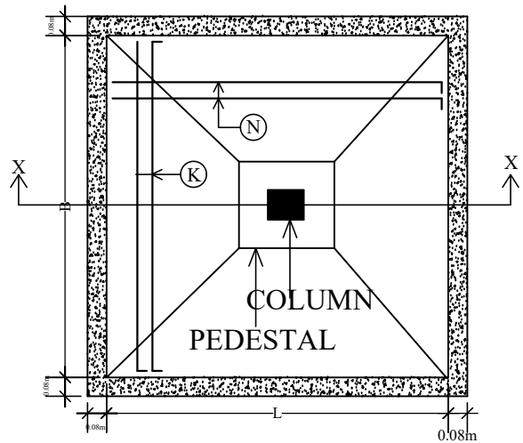
PLAN OF ISOLATED FOOTING
