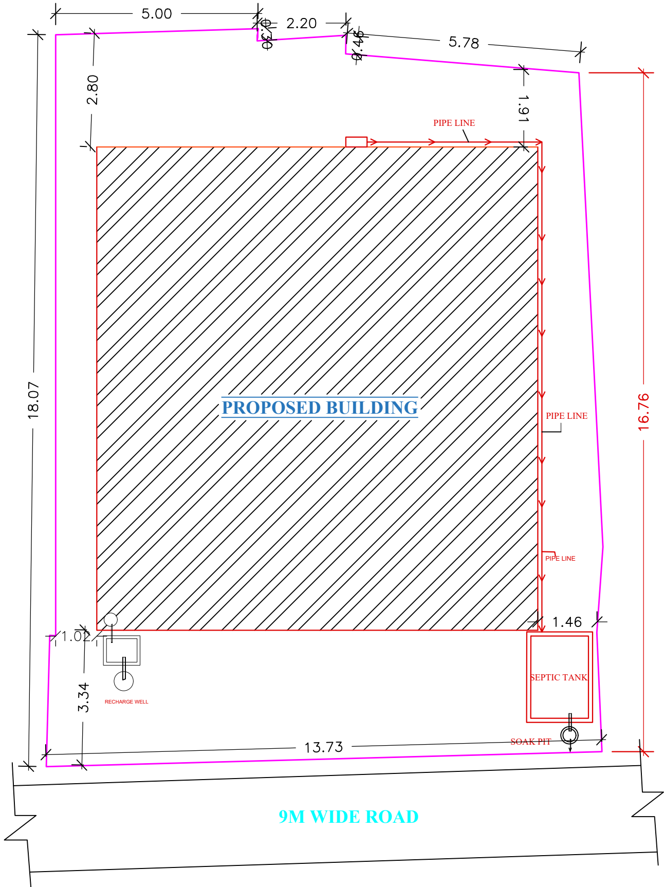
KEY PLAN EAST SIDE ROAD & FRONT
