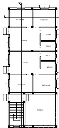
GROUND FLOOR PLAN SCALE: 1:100
