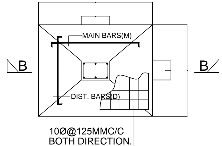
FOUNDATION PLAN OF CLOUMN
