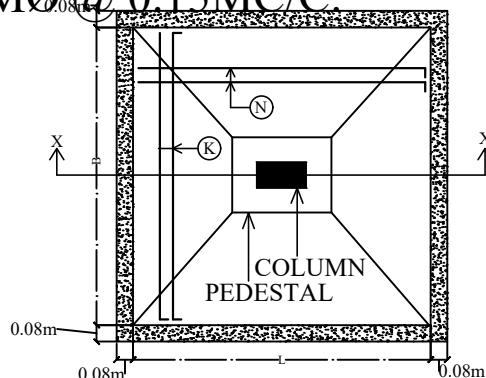
PLAN OF ISOLATED FOOTING
