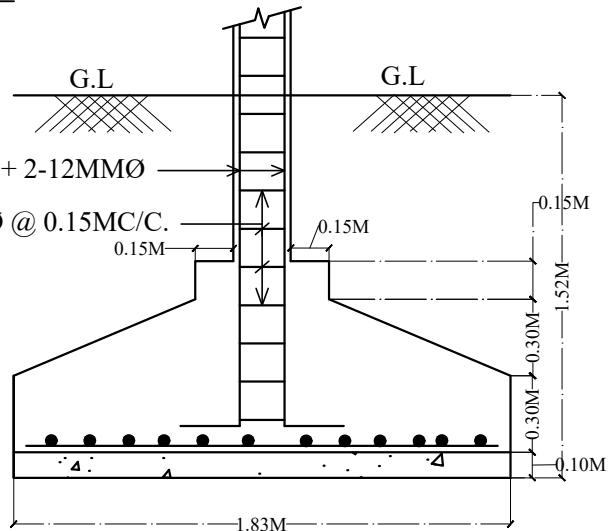
SECTION OF FOOTING
