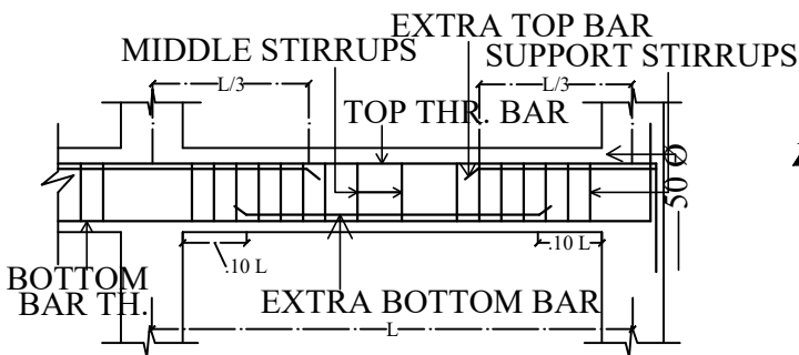
SECTION OF TYPICAL FLOOR BEAM
