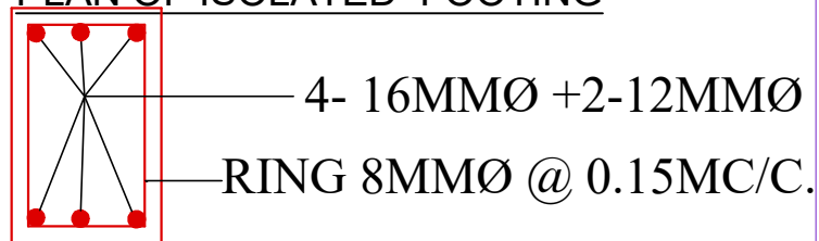
PLAN OF ISOLATED FOOTING
