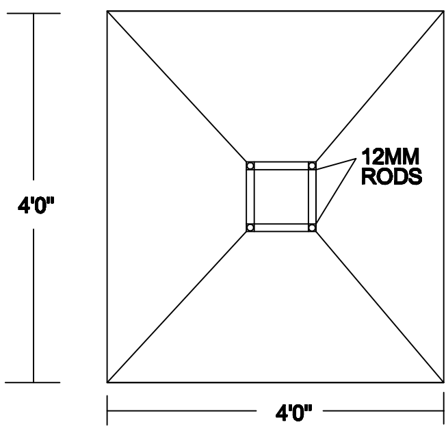
PLAN ( SCALE 1"=4' )
