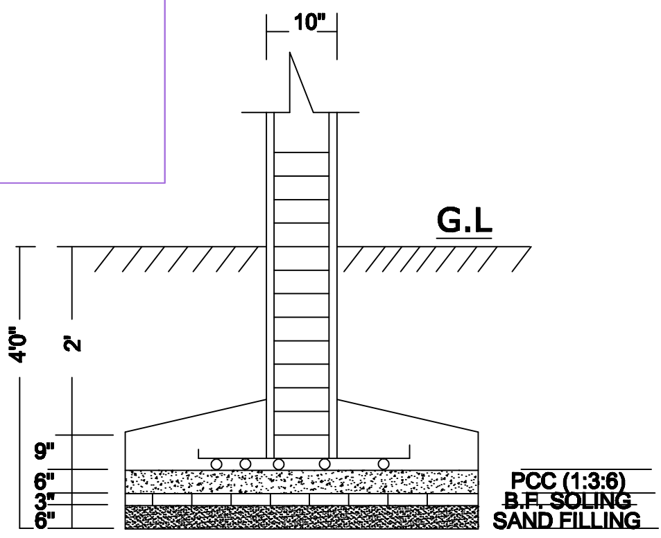
SECTION
