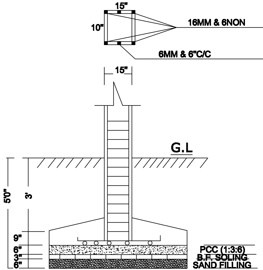
SECTION
