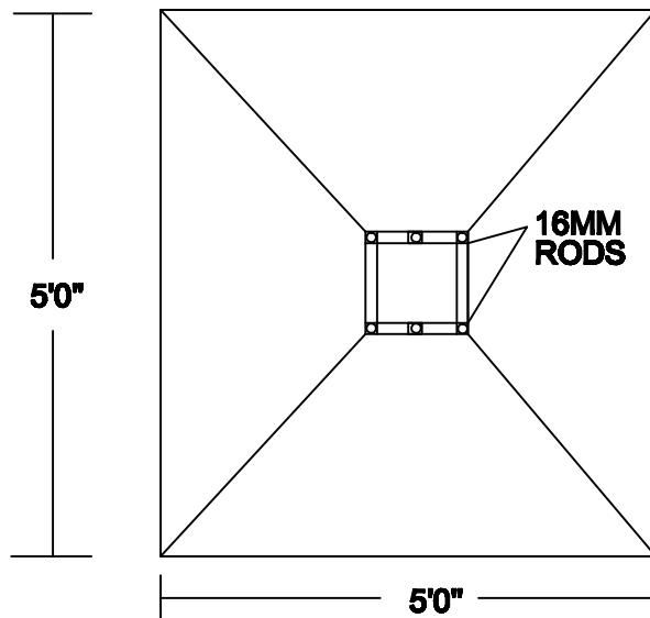
PLAN ( SCALE 1"=4' )
