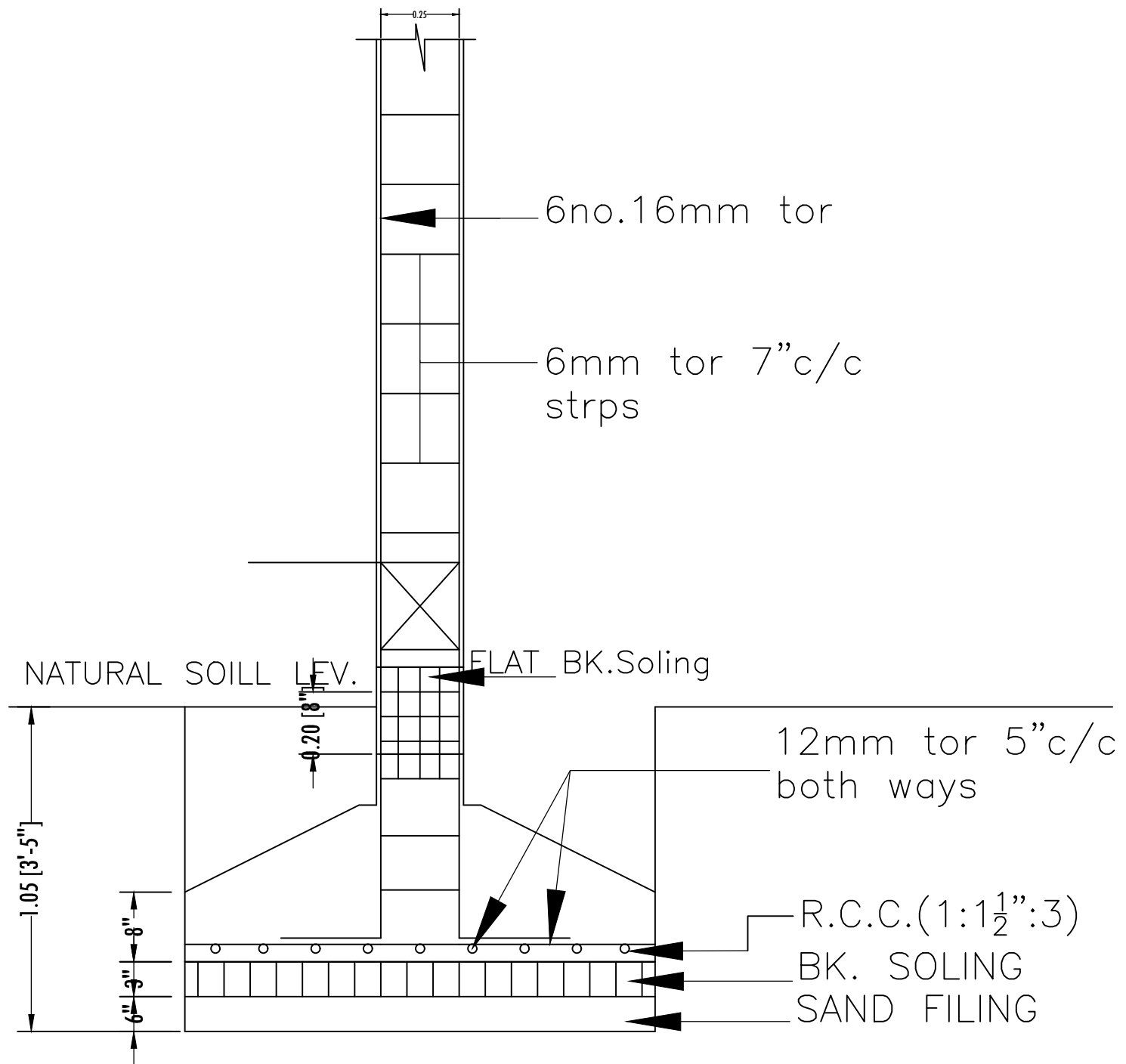
SEC. X-Y R.C.C. COLUMN FDN.DETAIL
