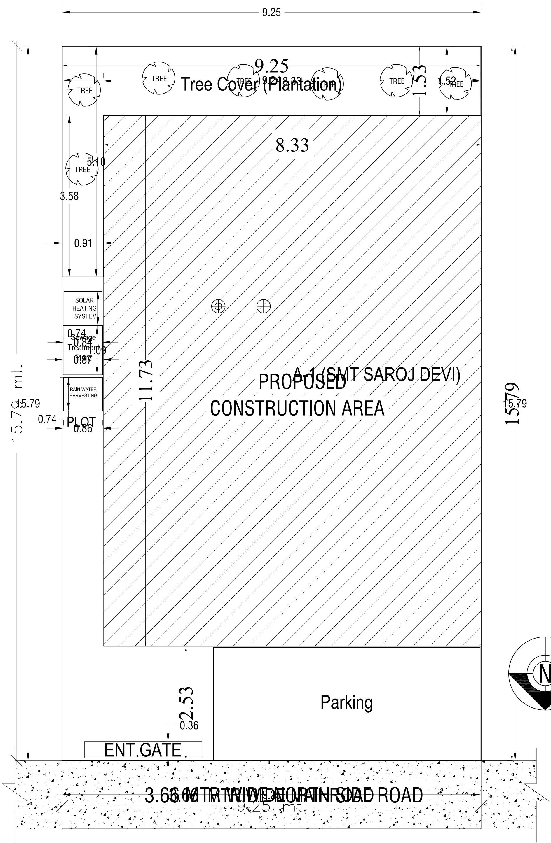
SITE PLAN
