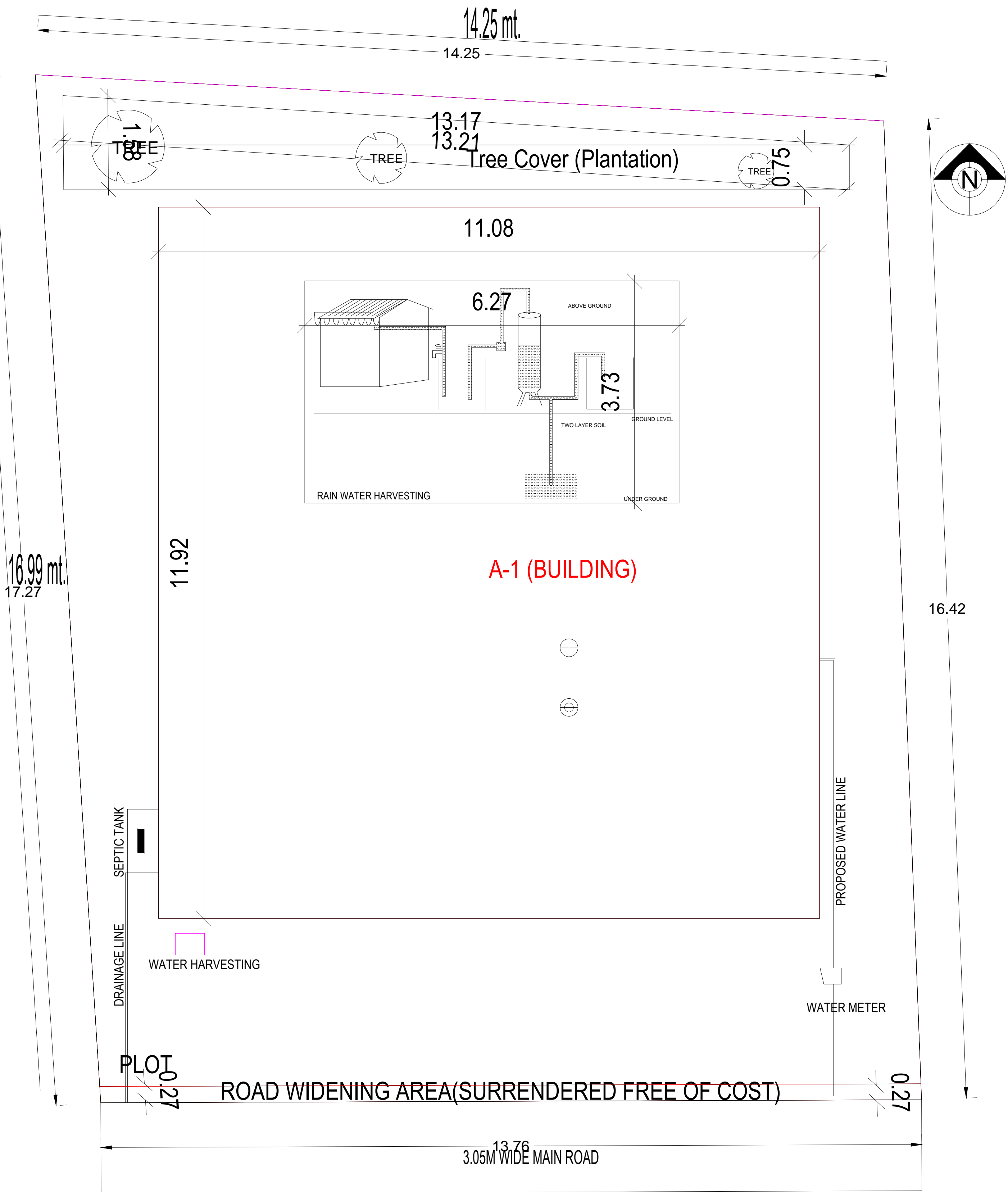
ROAD WIDENING LAYOUT PLAN
