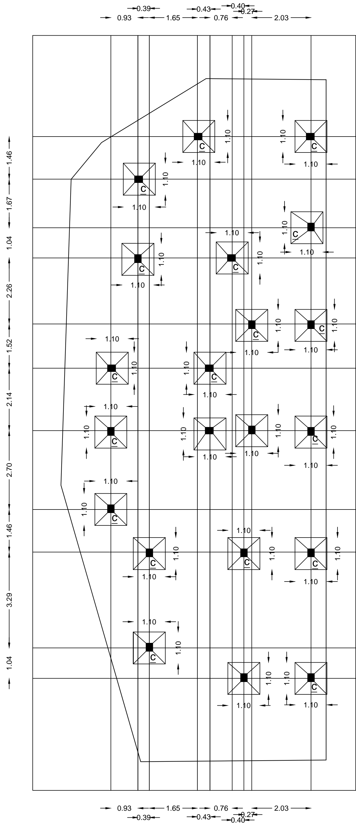
LAYOUT PLAN FOUNDATION AND COLUMN
