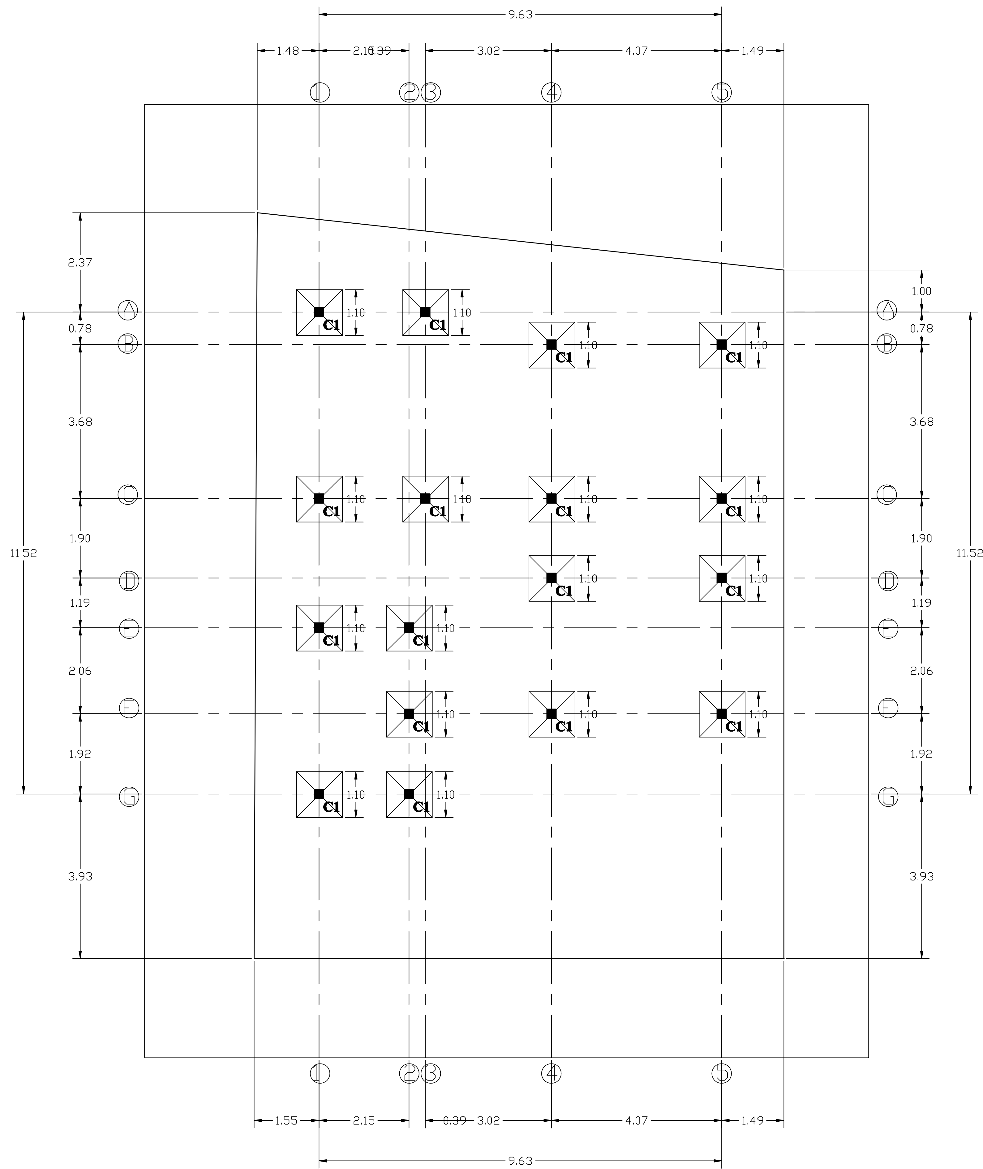
LAYOUT PLAN FOUNDATION AND COLUMN
