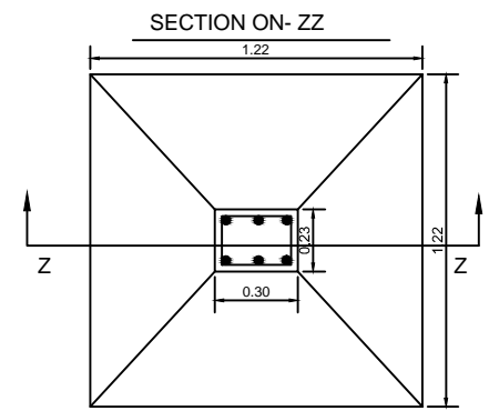
SECTION ON-ZZ PLAN *DETAILS OF COLUMN FOOTING SCALE :- 1" = 2'-0"
