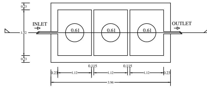
PLAN OF SEPTIC TANK SCALE:- 1"=4'-0"
