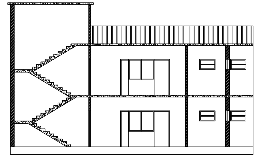
SECTION AT Y-Y SCALE- 1"=8'
