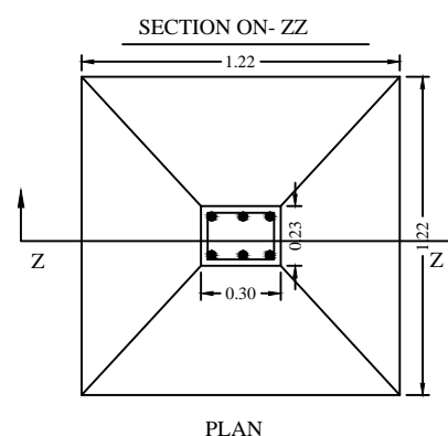
*DETAILS OF COLUMN FOOTING SCALE :- 1" = 2'-0"
