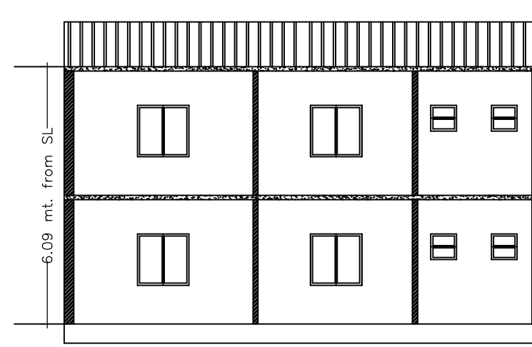
SECTION AT X-X SCALE- 1"=8'
