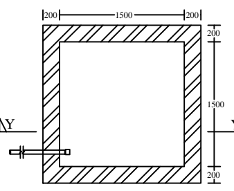
PLAN OF RECHARGE WELL (WATER HARVESTING) SCALE:- 1"=4'-0"
