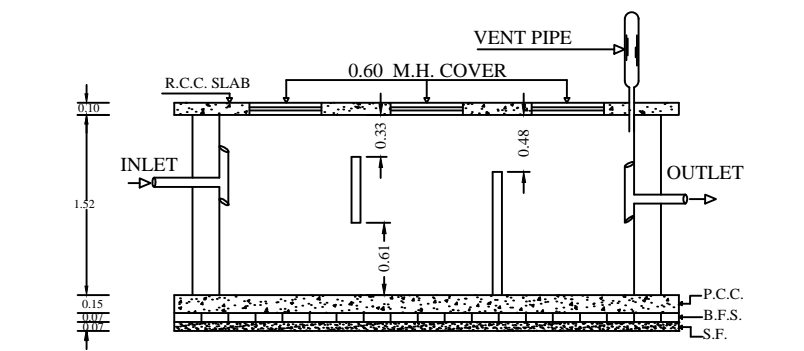
SECTION OF SEPTIC TANK SCALE:- 1"=4'-0"
