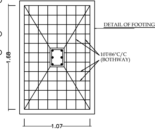
STRUCTURAL DETAILS Column & Footing
