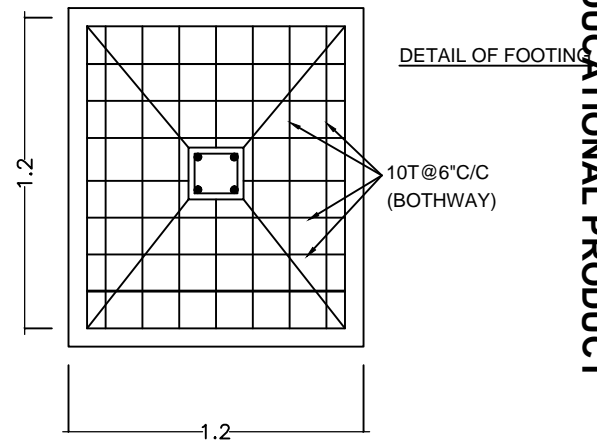
STRUCTURAL DETAILS Column & Footing
