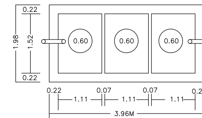
PLAN OF SEPTIC TANK (SCALE:-1IN. = 4FT.)
