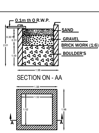
DETAIL'S OF WATER HARVESTING
