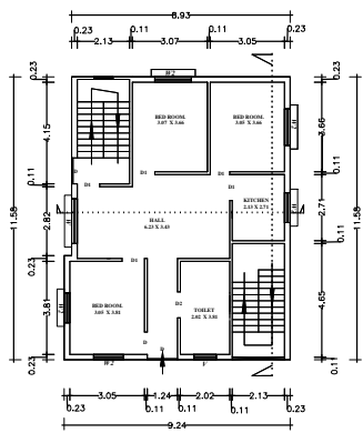
GROUND FLOOR PLAN SCALE = 1:2
