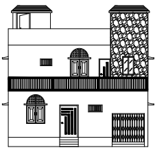
FRONT SIDE ELEVATION SCALE = 1:2
