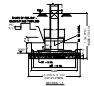
DETAILS OF COLUMN FOOTING
