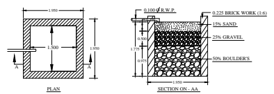
DETAILS OF WATER HARVESTING SCALE = 1:2
