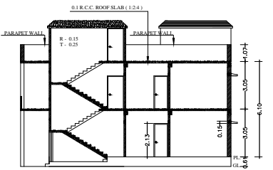
SECTION ON - YY SCALE = 1:2
