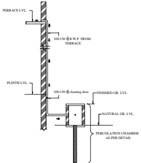
ROOF TOP RAIN WATER COLLECTION SYSTEM SCALE = 1:2
