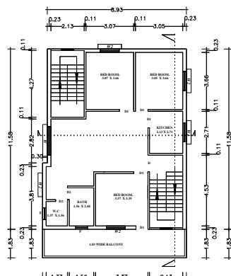
FIRST FLOOR PLAN SCALE = 1:2
