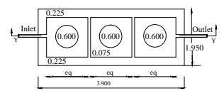
DETAILS OF SEPTIC TANK SCALE = 1:2
