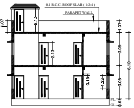
SECTION ON - XX SCALE = 1:2
