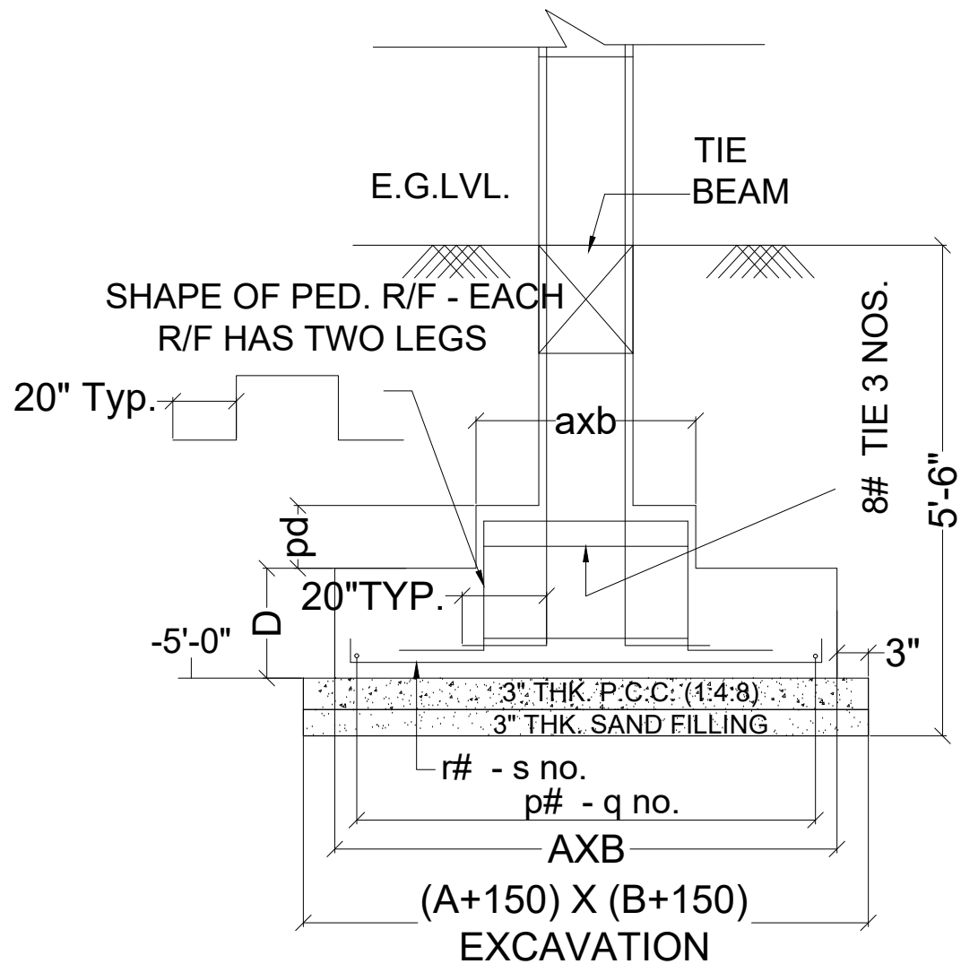
SECTION 1-1
