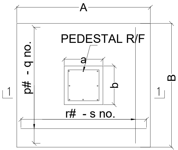
PLAN OF TYP. ISOLATED FOOTING
