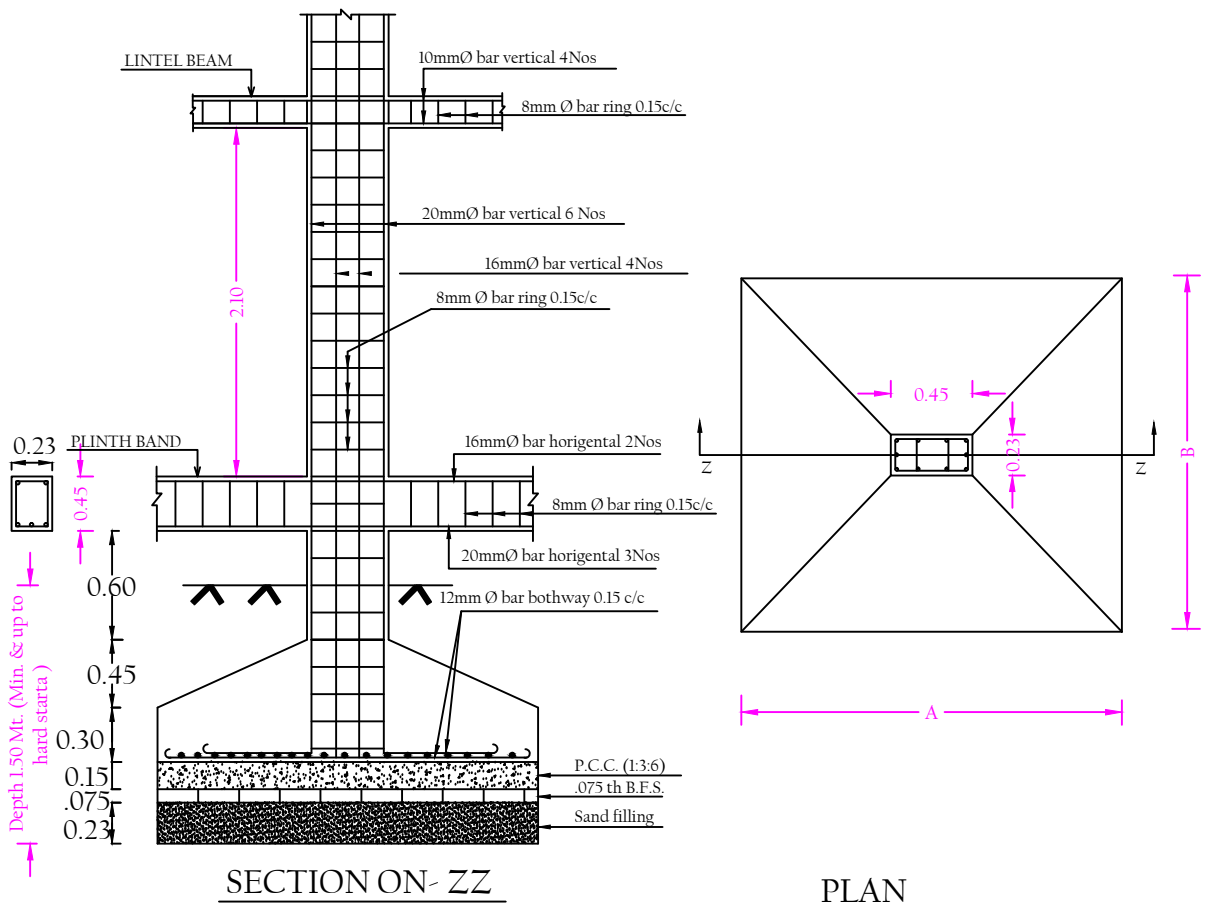
DETAILS OF TYPICAL COLUMN FOOTING Structure Detail
