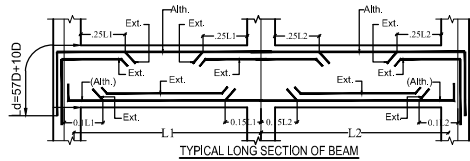
TYPICAL LONG SECTION OF BEAM
