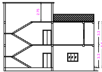
SECTION ON X-X
