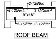
ROOF BEAM
