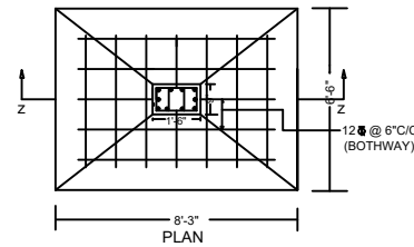
DETAIL OF COLUMNS
