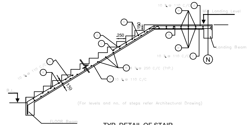
TYP. DETAIL OF STAIR
