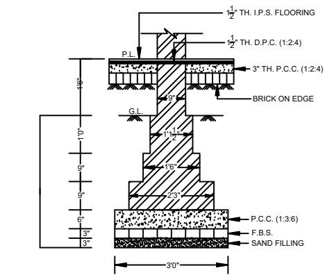
-:DETAIL OF BRICK FOUNDATION:-
