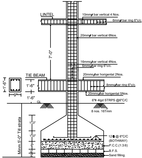
SECTION ON Z-Z
