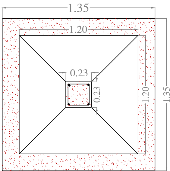
FOUNDATION PLAN
