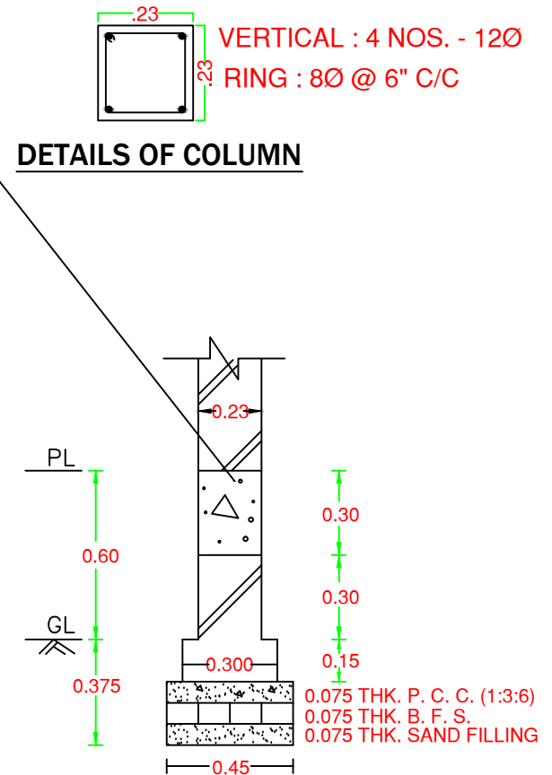
FOUNDATION DETAILS OF WALL
