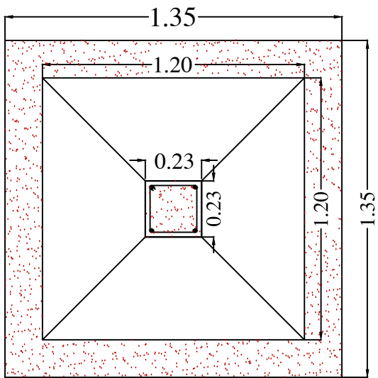
FOUNDATION PLAN
