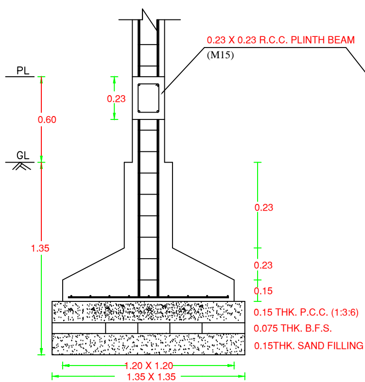
FOUNDATION DETAILS OF COLUMN
