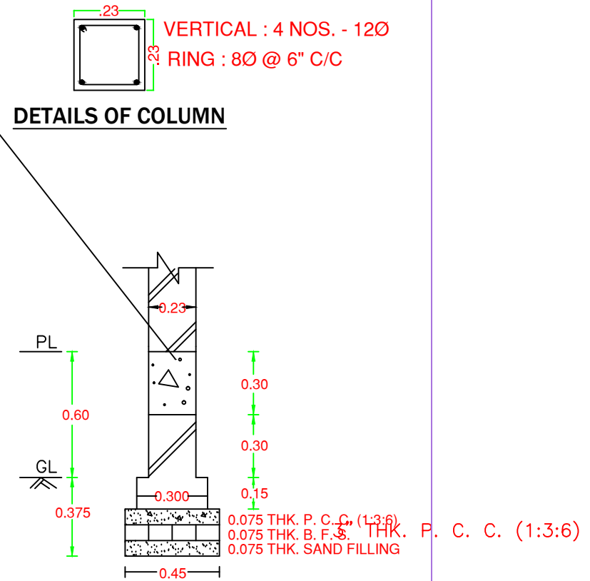
FOUNDATION DETAILS OF WALL
